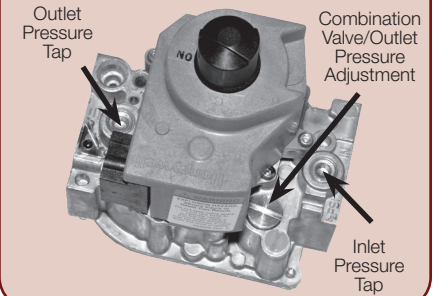
Figure 4: Combined Regulator Valve
