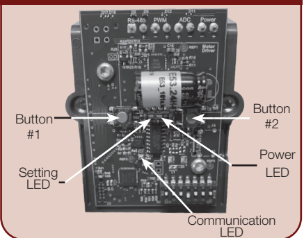
Figure 5: EXA Modulating Gas Valve (with cover removed)
