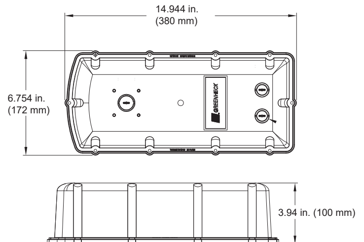
NEMA cover
