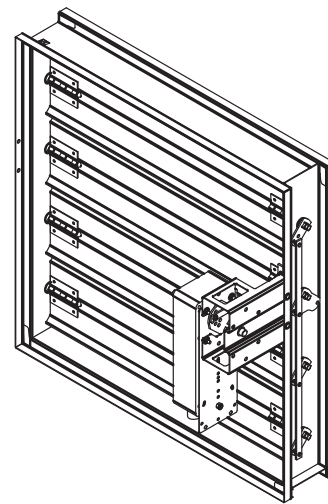
Non jackshafted internal (right) includes actuator and mounting hardware. Actuator is in the airstream.
