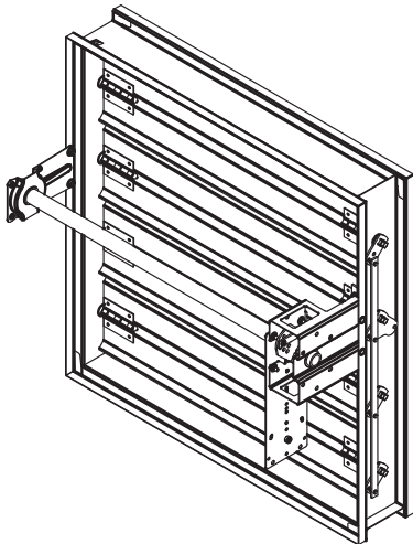
Jackshaft internal (right) includes actuator mounting bracket
