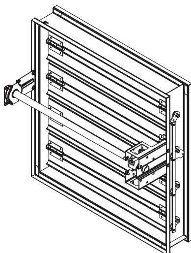
Jackshaft internal (right) includes crankarm assembly and jackshaft, no actuator mounting hardware. Actuator is in the airstream.
