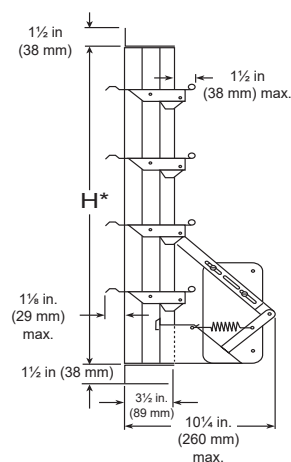
Model WD-220 Flange Opposite Motor
