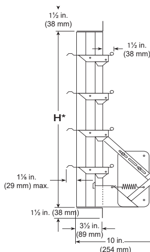
Model WD-210 Flange on Motor Side
