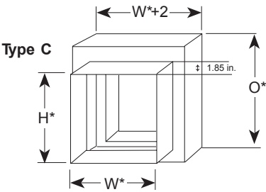
Overall Damper Dimensions
