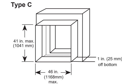
Maximum Single Section Dimensions
