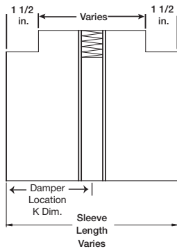
Type B2 side view
