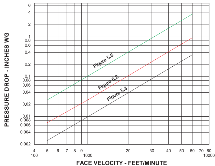
Leakage 36 x 36 in. (914mm x 914mm) Damper (based on 5 in. lb/ft 2 of torque)
