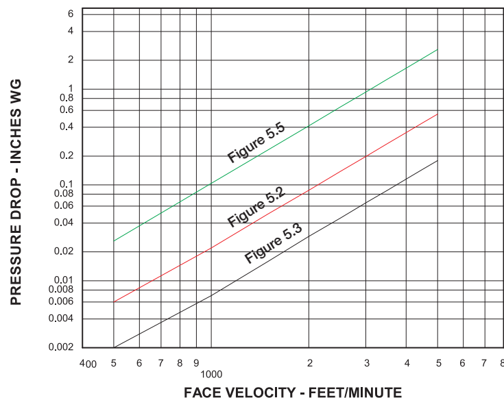
Pressure Drop 36 x 36 in. Damper (914 mm x 914 mm) VELOCITY VS. PRESSURE DROP
