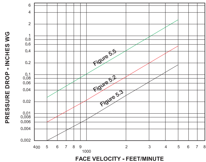
VELOCITY VS. PRESSURE DROP
