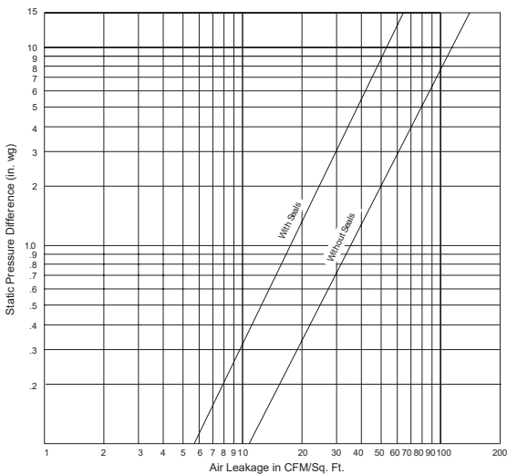
Leakage 36 x 36 in. (914 mm x 914 mm) Damper (based on 5 in. lb/ft 2 of torque)
