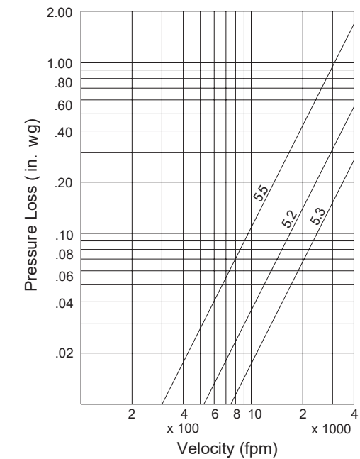
Pressure Drop 36 x 36 in. Damper (914 mm x 914 mm)
