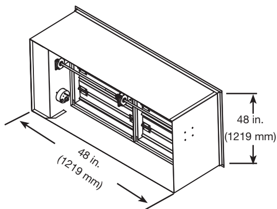
Double Section
