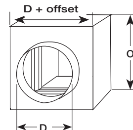
Overall Damper Dimensions Type R
