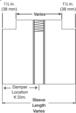
Type B2 Side View
