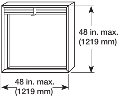
Type A - Maximum Dimensions
