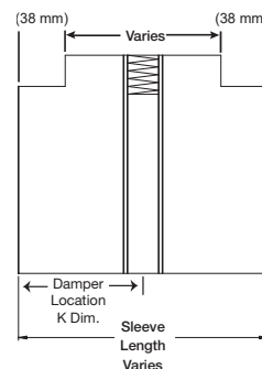
Type B2 side view
