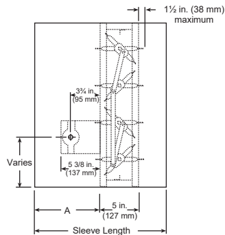
Sleeve
