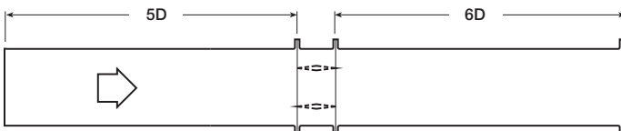
AMCA Figure 5.3
