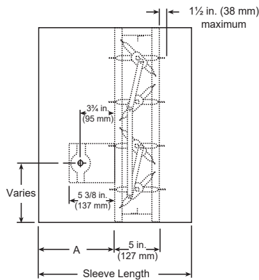
Sleeve
