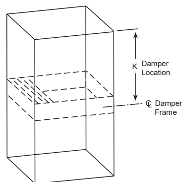
HORIZONTAL MOUNT
