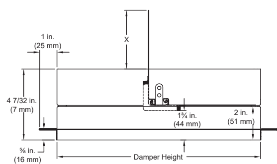
Grille Mount
