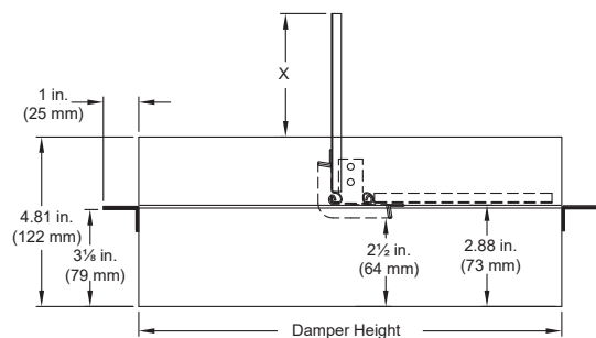
Duct Mount
