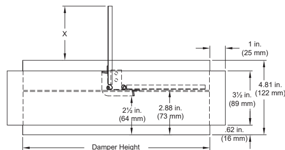
CRD-1WT with Insulation Band
