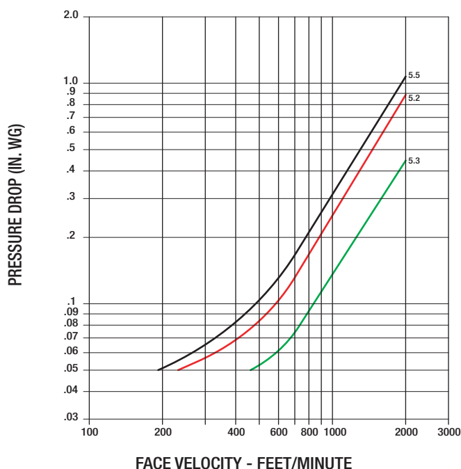
Damper Size 36 in. x 36 in. (914 mm x 914 mm)
