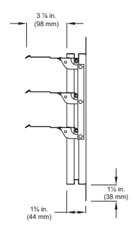
BD-300 Flange on Intake
