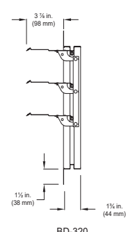
BD-320 Flange on Discharge
