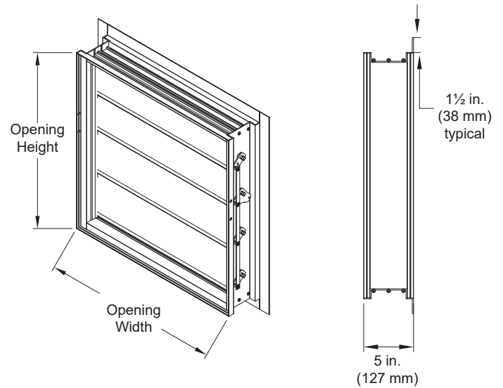
Reverse Flange
