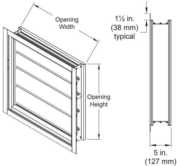
Single Flange
