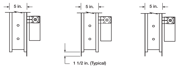
Single Flange
