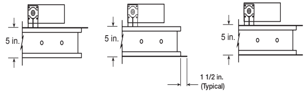
Single Flange
