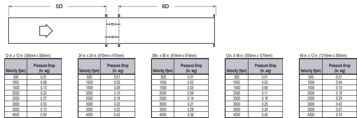
AMCA Figure 5.5
