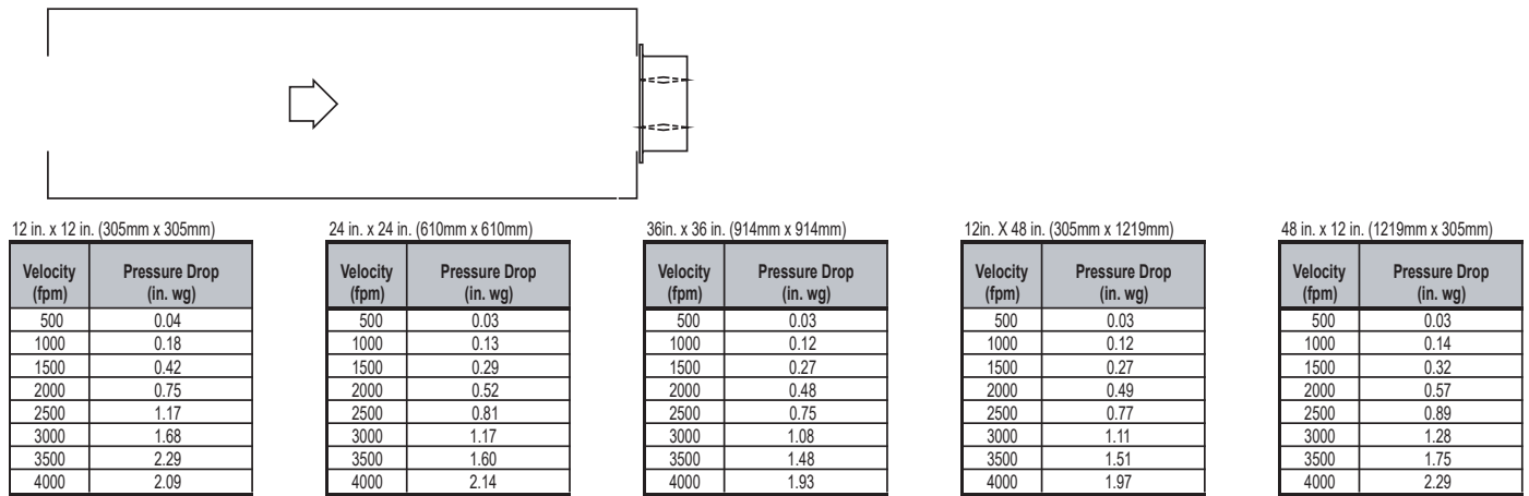
AMCA Figure 5.5
