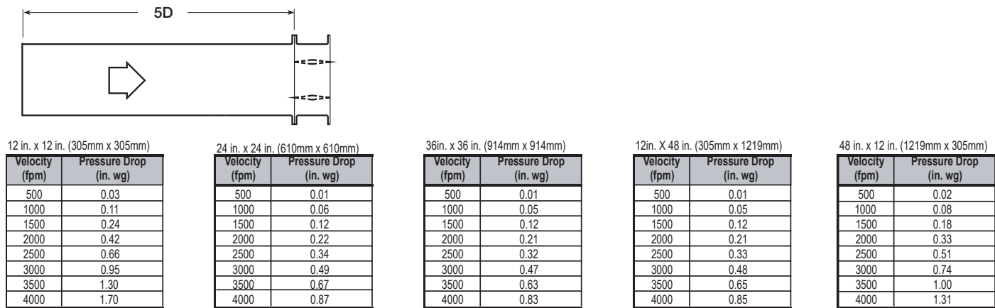
AMCA Figure 5.3
