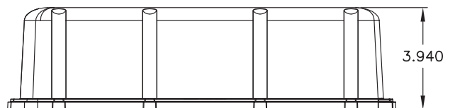
NEMA cover
