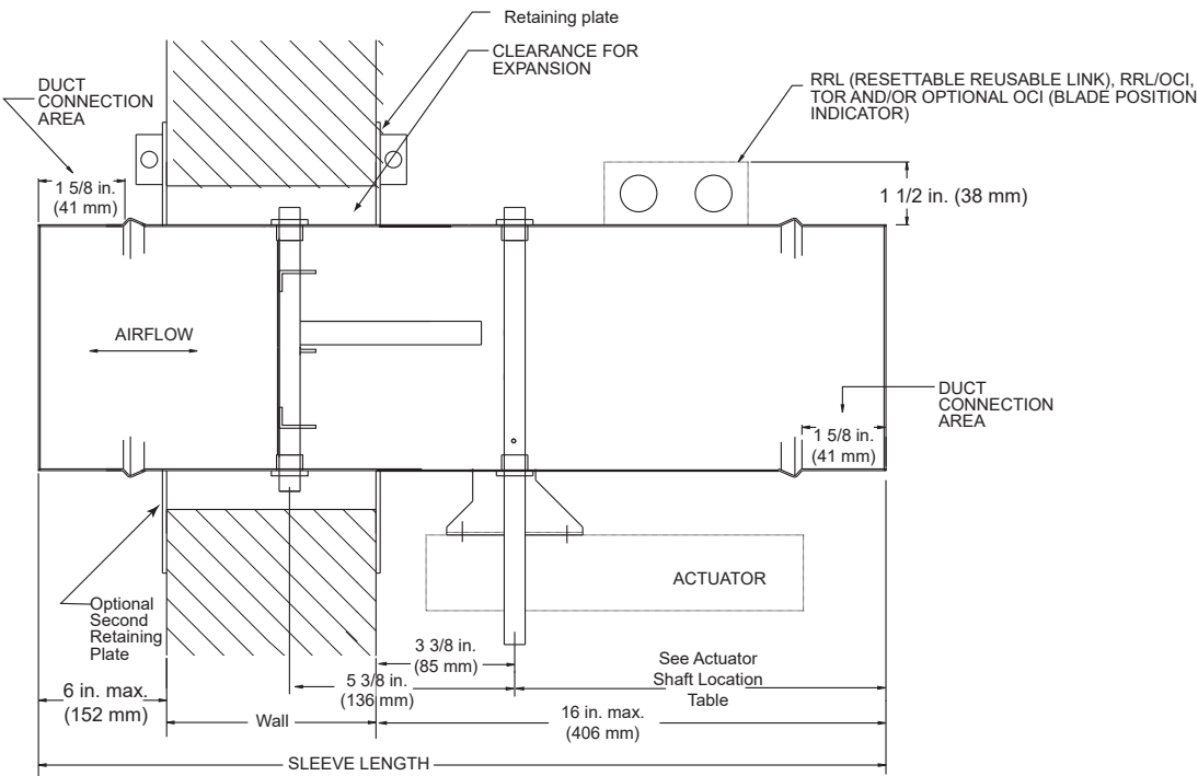
TOP VIEW OF DAMPER
