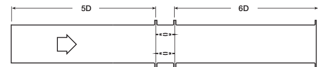
AMCA Figure 5.3
