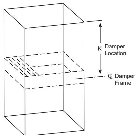
HORIZONTAL MOUNT
