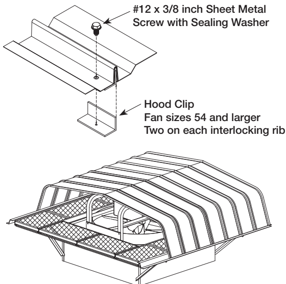
Detail 1B
