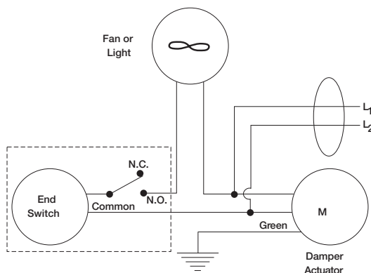
Wiring Illustration
